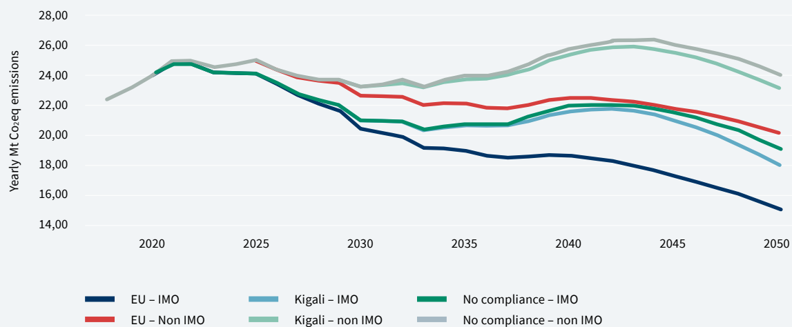
Figure 13. Yearly emissions of average scenarios and their variability
